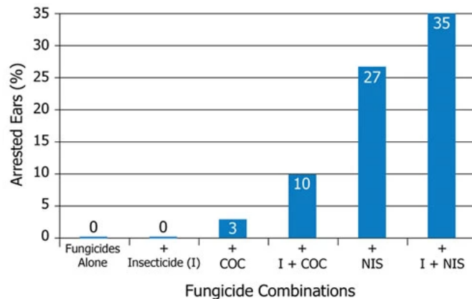
Figure 3. Corn ear response to foliar treatments applied alone or with crop oil concentrate or nonionic surfactant (Nielsen et al., 2008).
