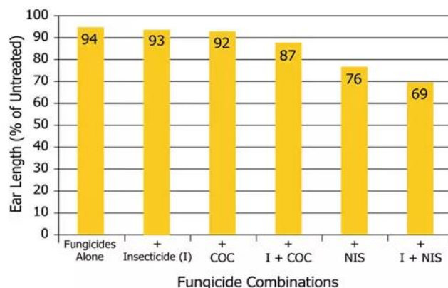
Figure 4. Corn ear length associated with foliar treatments applied alone or with crop oil concentrate or nonionic surfactant (Nielsen et al., 2008).
