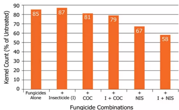
Figure 5. Corn kernel number associated with foliar treatments applied alone or with crop oil concentrate or nonionic surfactant (Nielsen et al., 2008).
