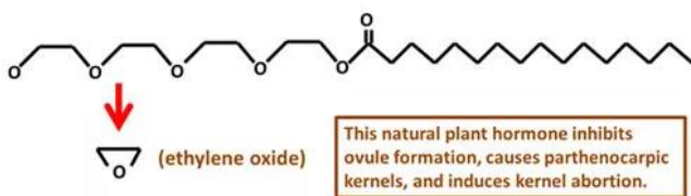
Figure 9. Ethylene oxide is one of the breakdown products of nonionic surfactant in plants.
